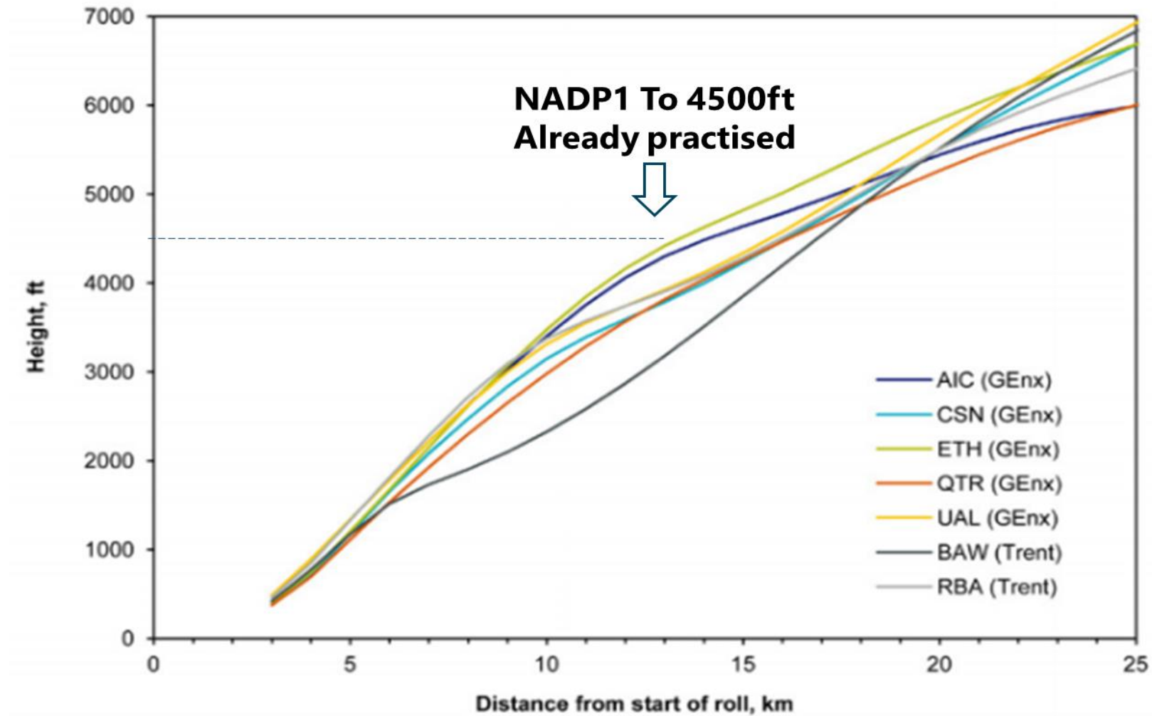
Figure 9 Comparison of average 787 departure height profiles by airline
