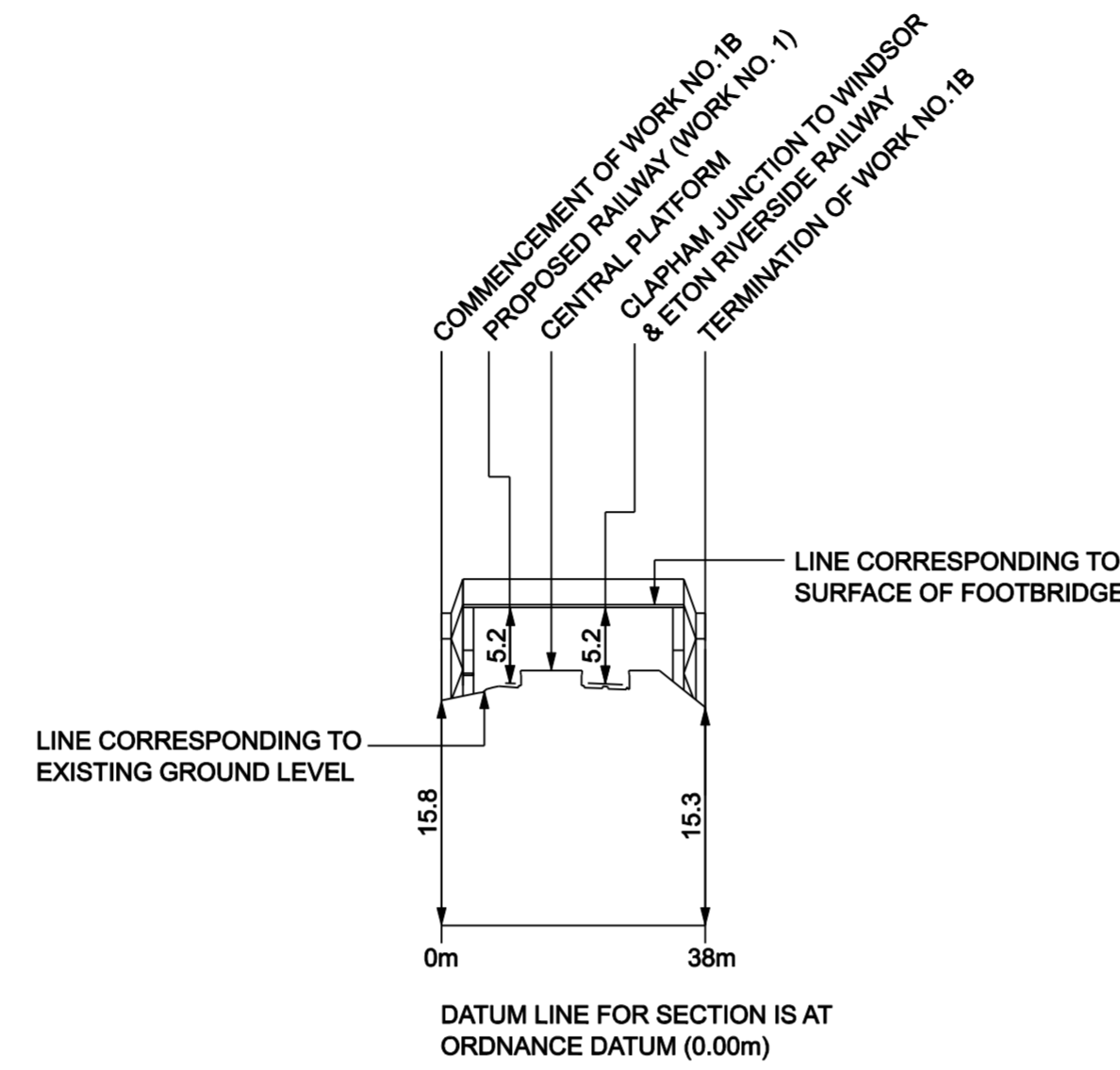
WORK NO. 1B TEMPORARY FOOTBRIDGE
