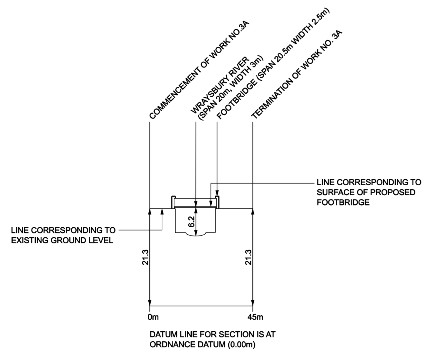
WORK NO. 3A FOOTBRIDGE
