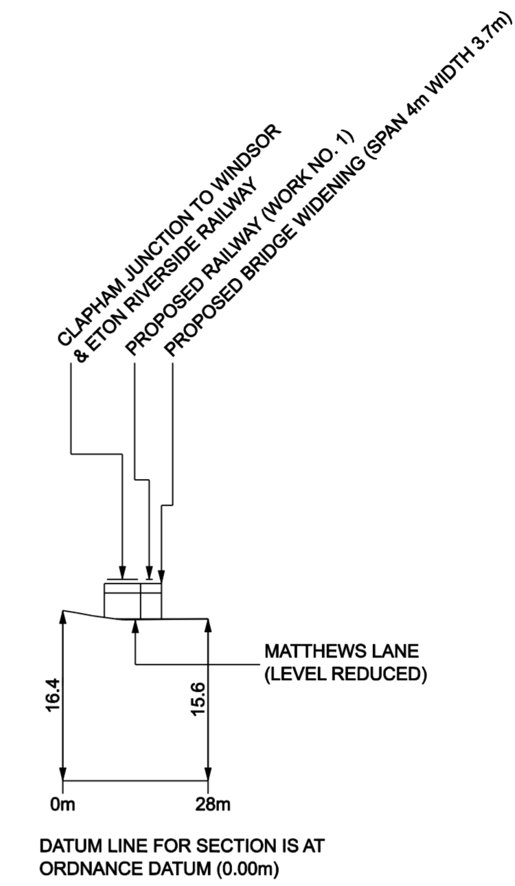
WORK NO. 1C BRIDGE WIDENING
