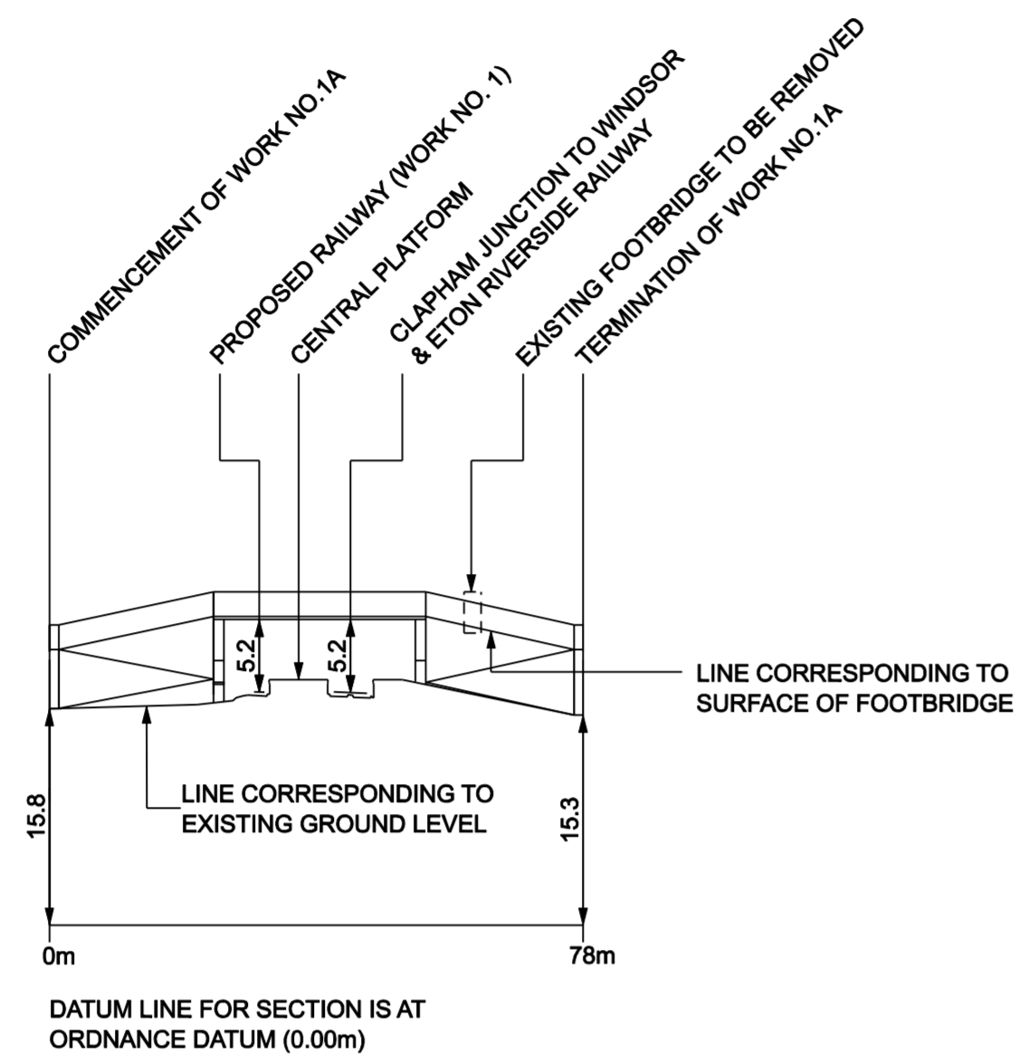
WORK NO. 1A FOOTBRIDGE
