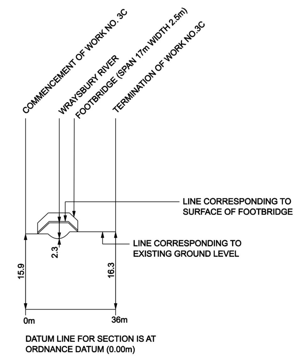
WORK NO. 3C BRIDGE
