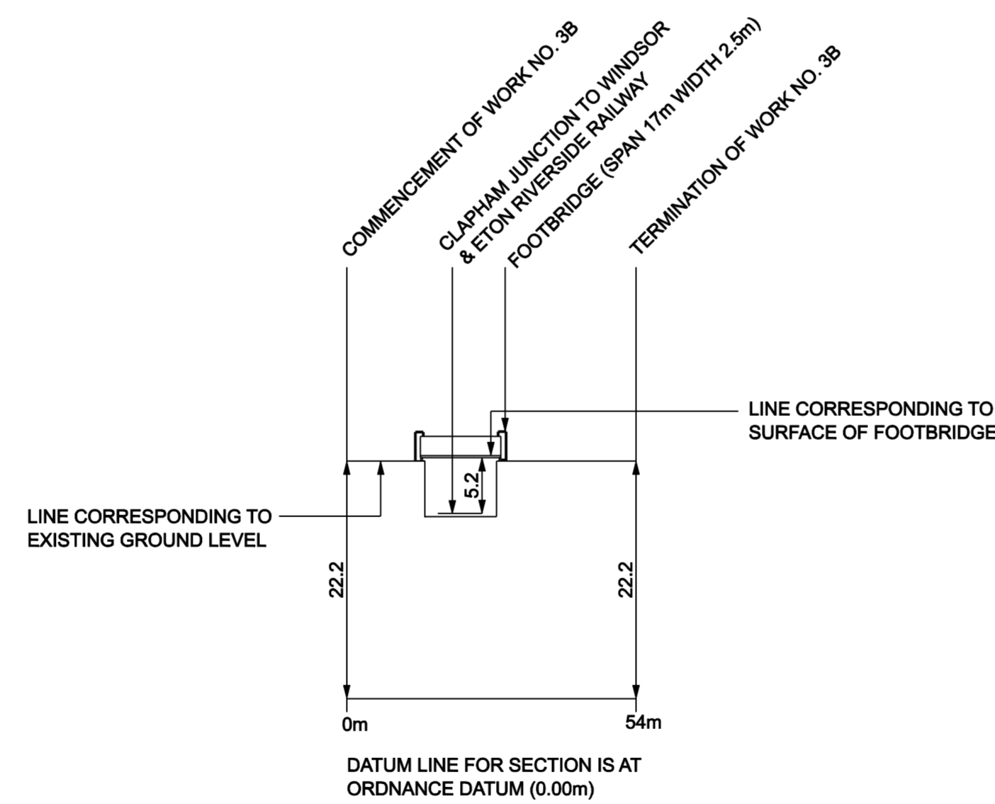
WORK NO. 3B FOOTBRIDGE
